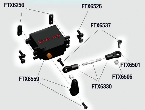
Steering Assembly
